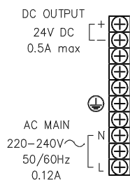
Terminal block
